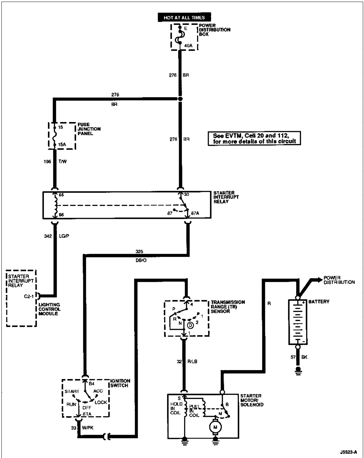
Starter System--1996 Town Car
